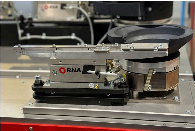
Typical application: PARU-Mini XS with orienting device
