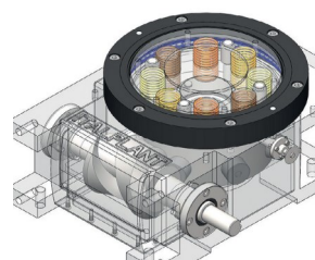
ADJUSTABLE TRANSMISSION TORQUE WITH SAFETY OUTPUT TORQUE LIMITER
