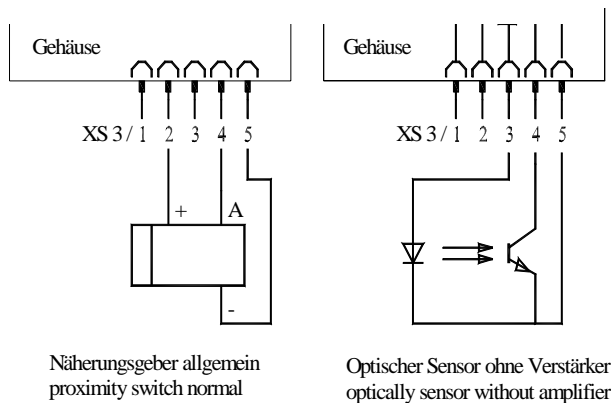
Fig.: Connecting diagram for direct sensors
